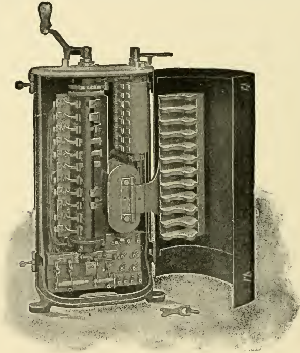
Fig. 52. K-10 Controller
